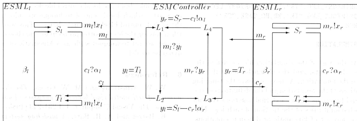
Figure 3: The system actors || controller.
